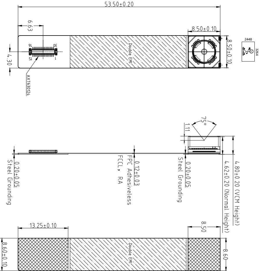
TOP VIEW
